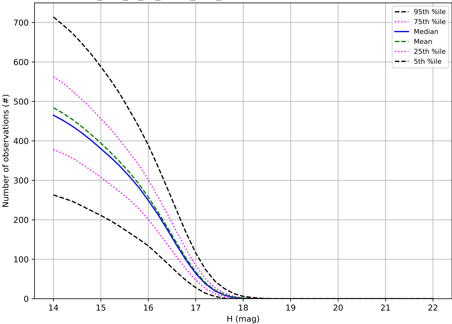
too_elab_r8_d3_ugrizy_v3.4_10yrs: Number of observations Trojan
