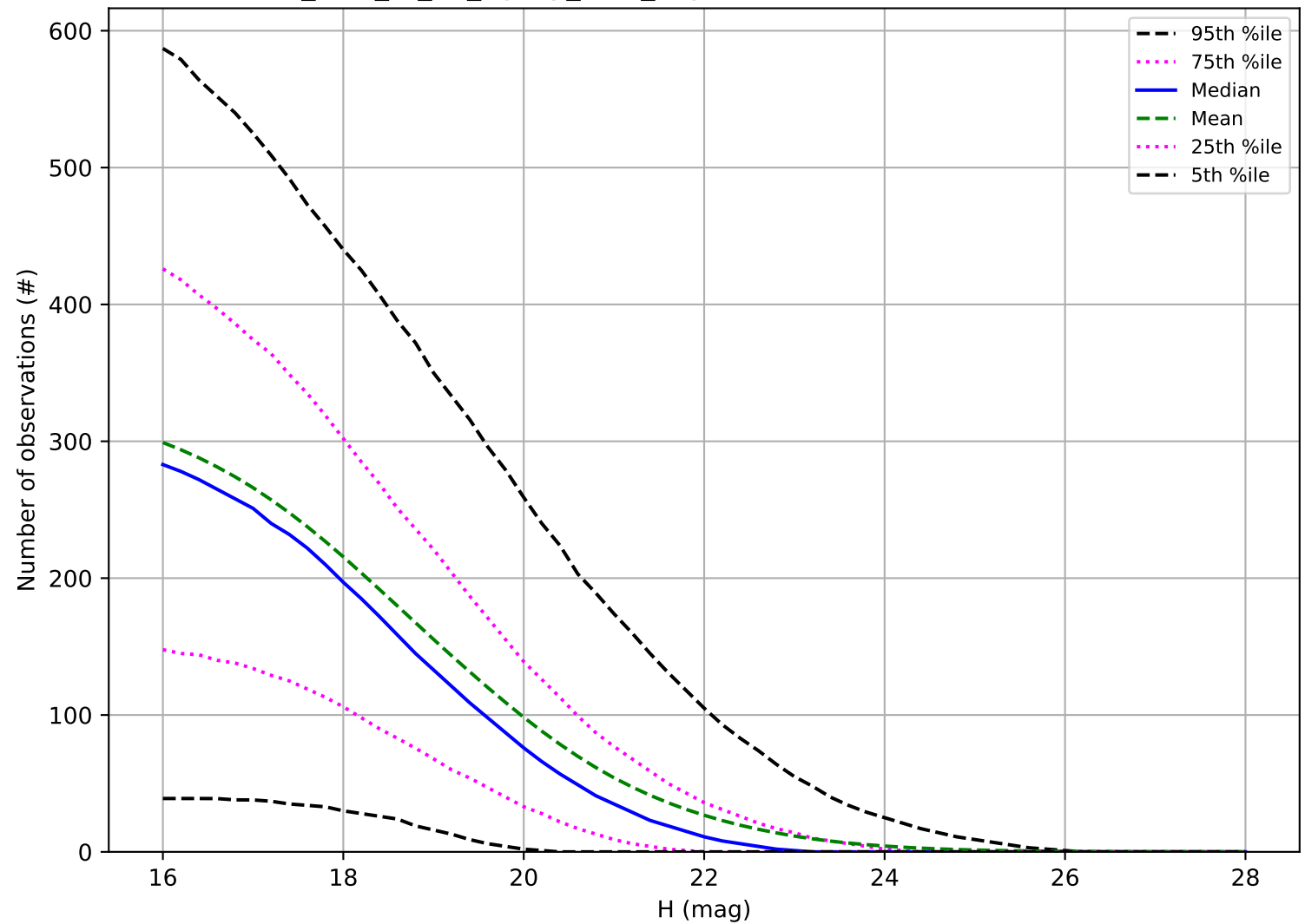
too_elab_r8_d3_ugrizy_v3.4_10yrs: Number of observations PHA
