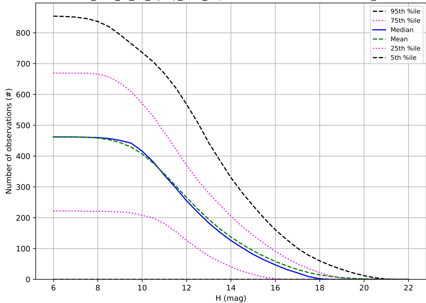
too_elab_r8_d3_ugrizy_v3.4_10yrs: Number of observations OCC_r5
