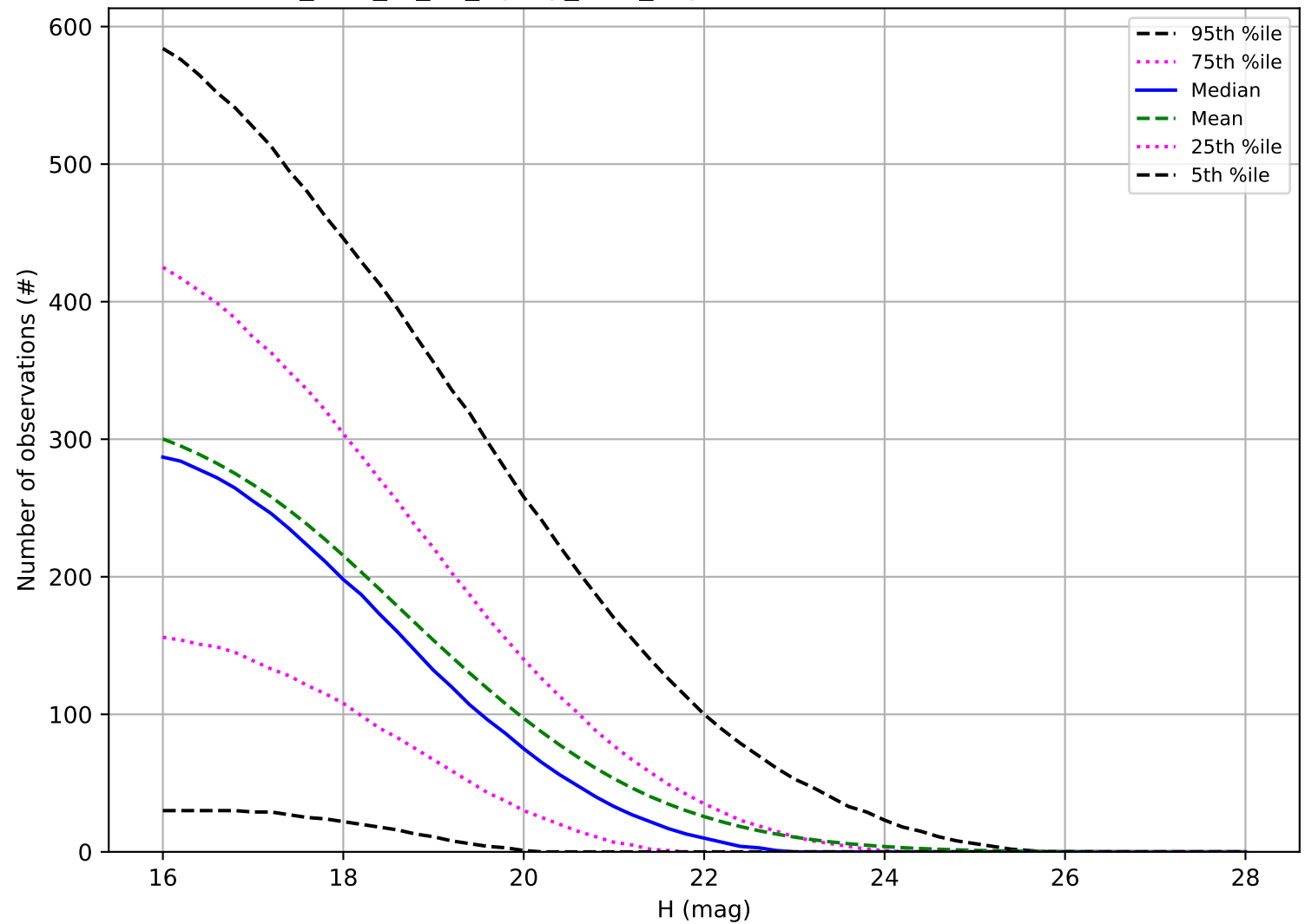
too_elab_r8_d3_ugrizy_v3.4_10yrs: Number of observations NEO
