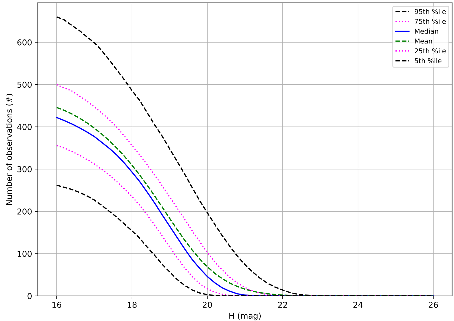
too_elab_r8_d3_ugrizy_v3.4_10yrs: Number of observations MBA
