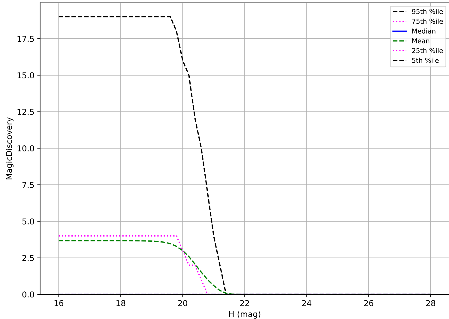
too_elab_r8_d3_ugrizy_v3.4_10yrs: Vatira 6 detections in 60 nights detection loss
