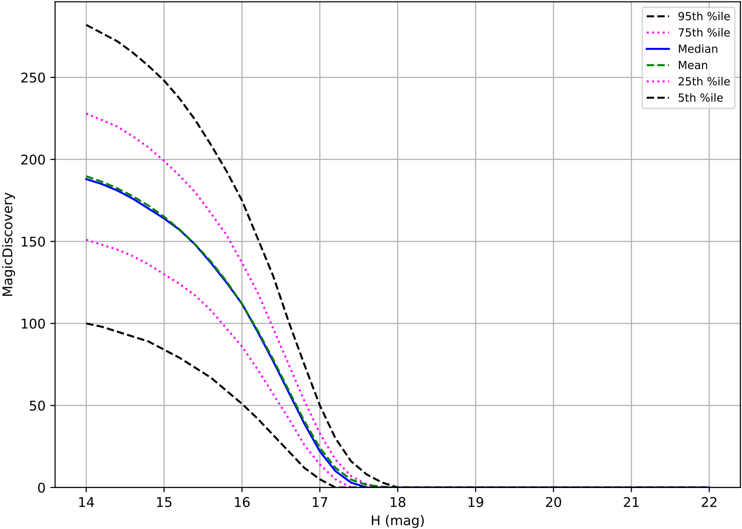
too_elab_r8_d3_ugrizy_v3.4_10yrs: Trojan 6 detections in 60 nights detection loss
