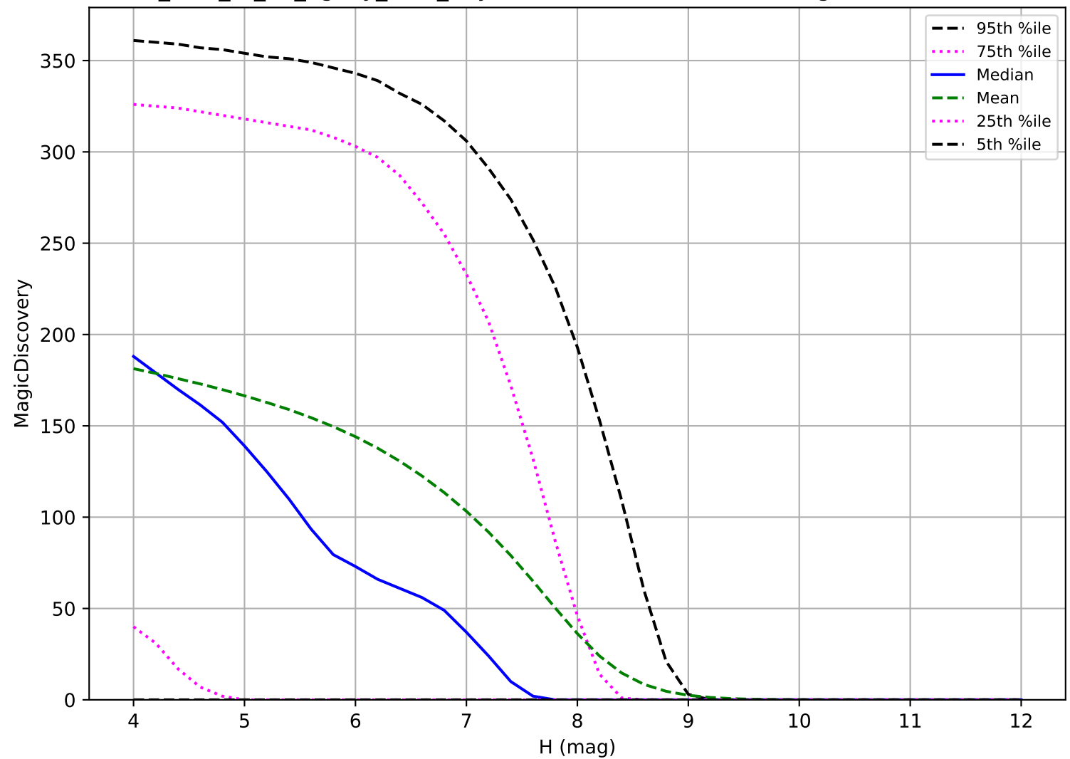
too_elab_r8_d3_ugrizy_v3.4_10yrs: TNO 6 detections in 60 nights detection loss
