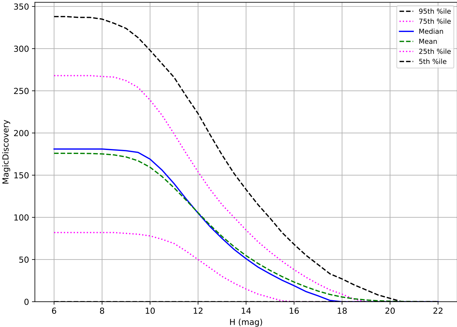
too_elab_r8_d3_ugrizy_v3.4_10yrs: OCC_r5 6 detections in 60 nights detection loss
