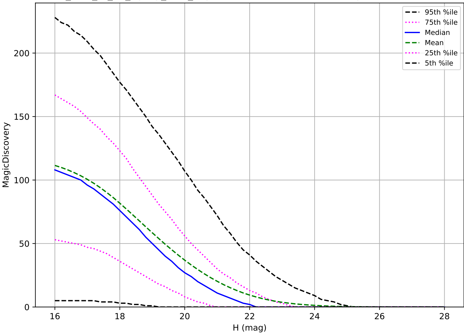
too_elab_r8_d3_ugrizy_v3.4_10yrs: NEO 6 detections in 60 nights detection loss
