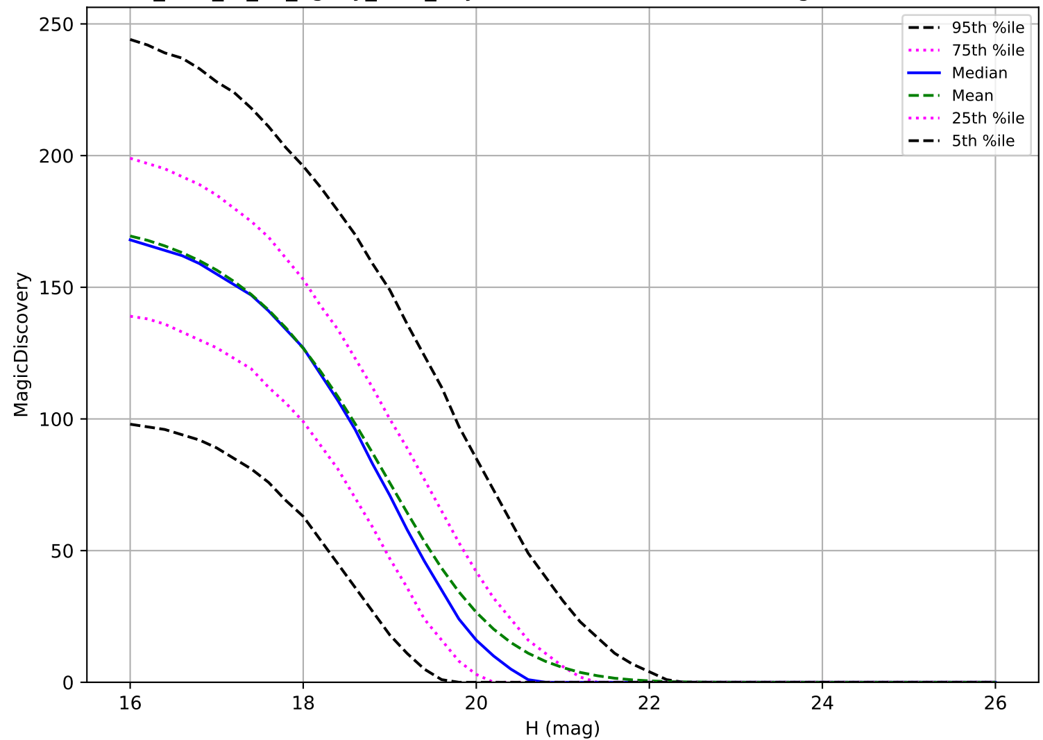
too_elab_r8_d3_ugrizy_v3.4_10yrs: MBA 6 detections in 60 nights detection loss
