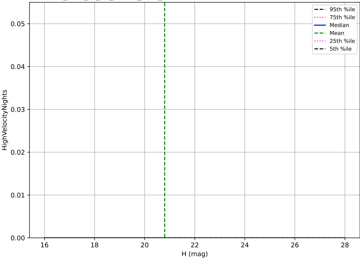
too_elab_r8_d3_ugrizy_v3.4_10yrs: Vatira High velocity pair detection loss
