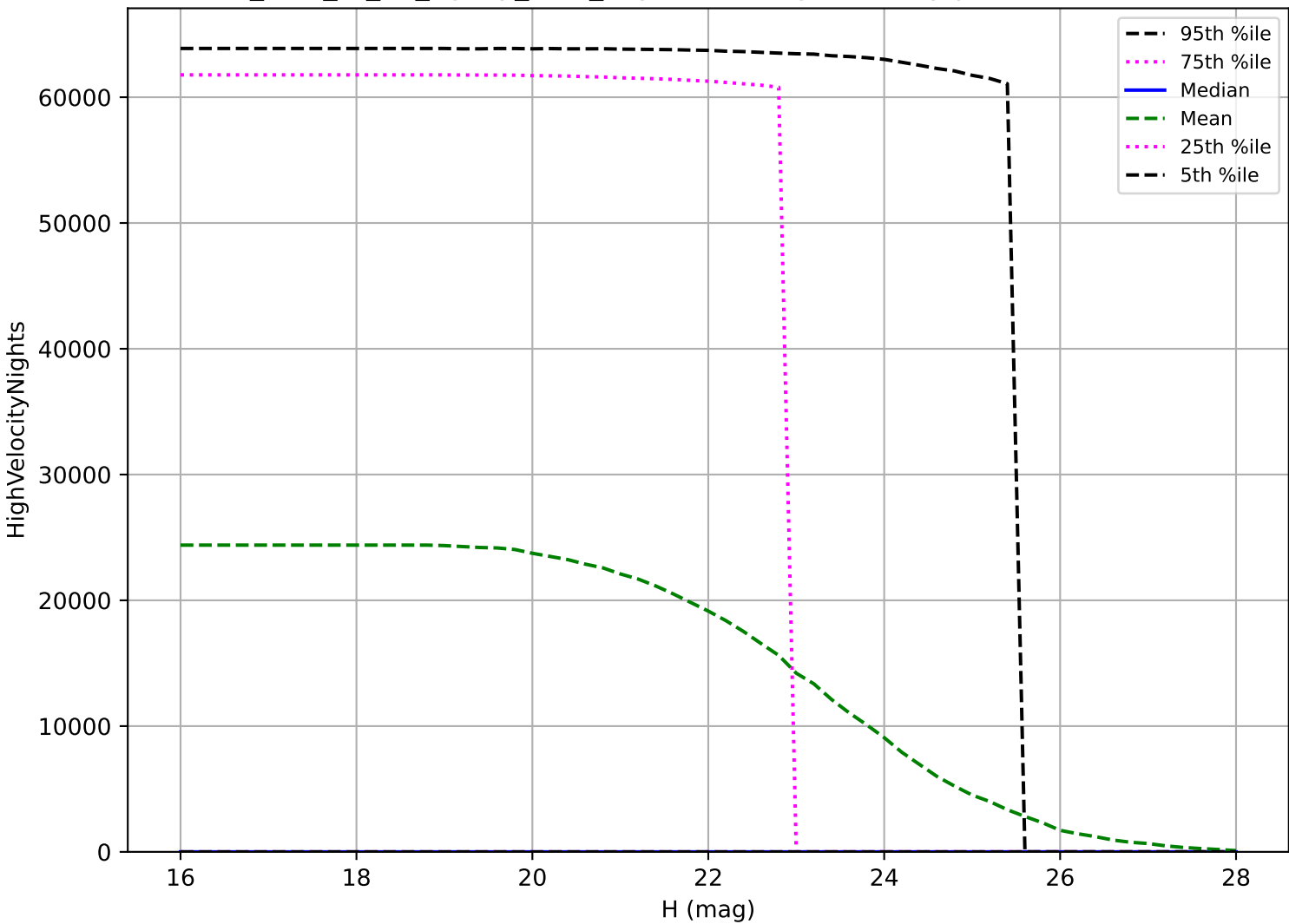
too_elab_r8_d3_ugrizy_v3.4_10yrs: PHA High velocity pair detection loss
