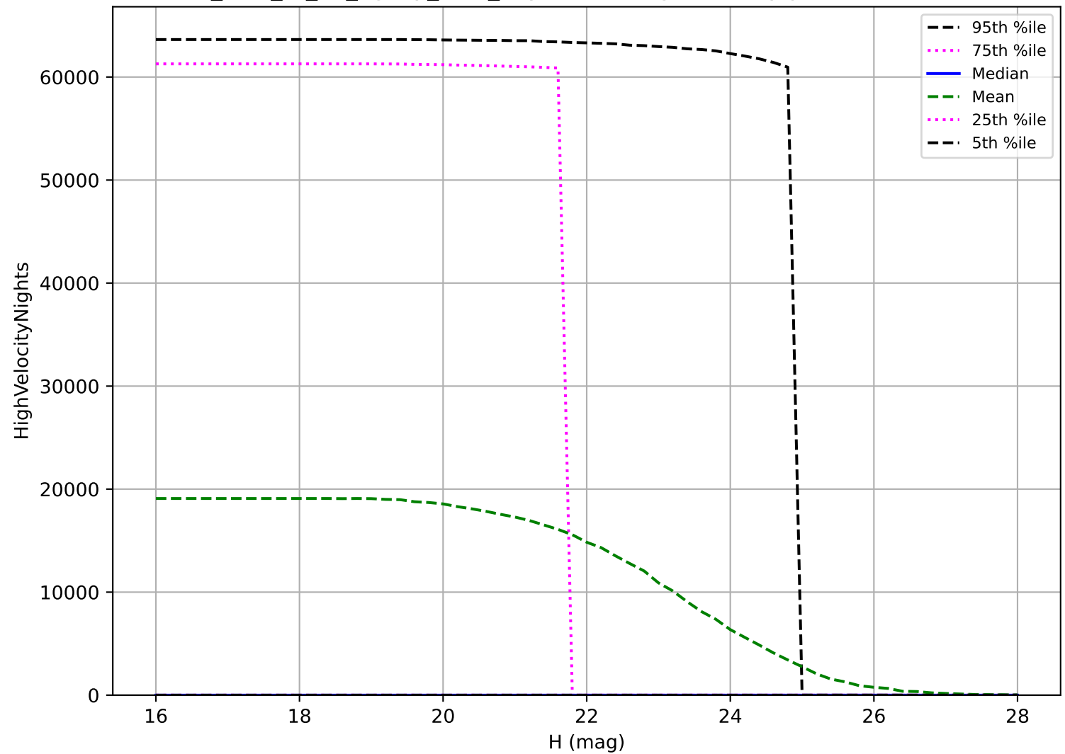
too_elab_r8_d3_ugrizy_v3.4_10yrs: NEO High velocity pair detection loss
