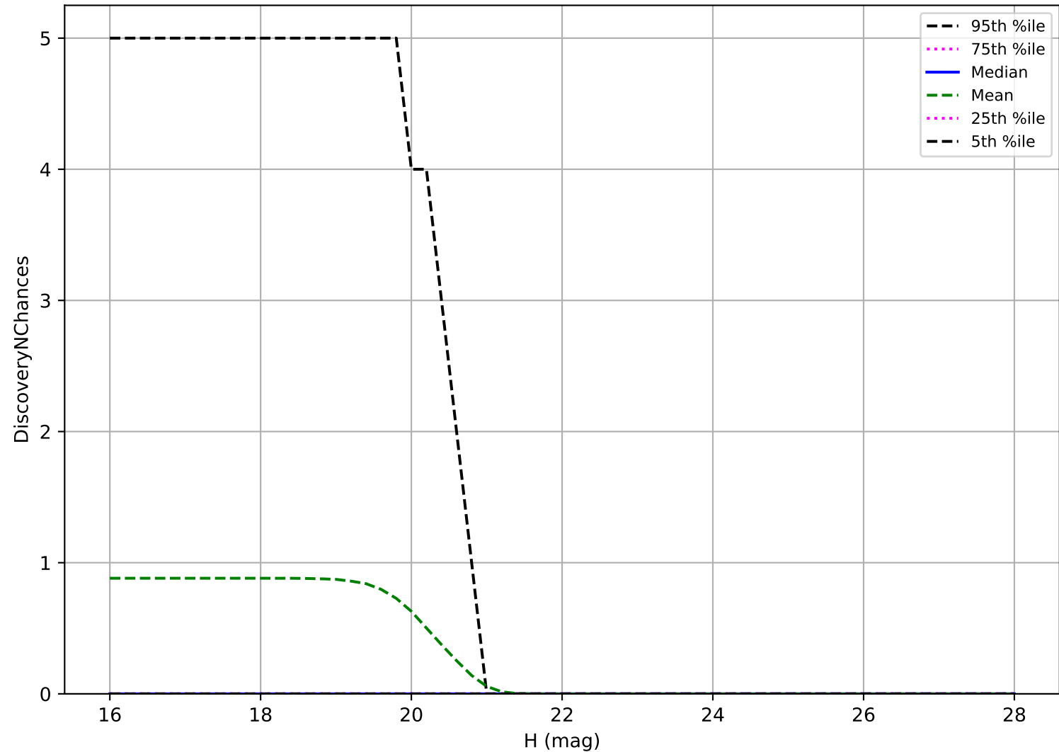
too_elab_r8_d3_ugrizy_v3.4_10yrs: Vatira 3 pairs in 15 nights detection loss
