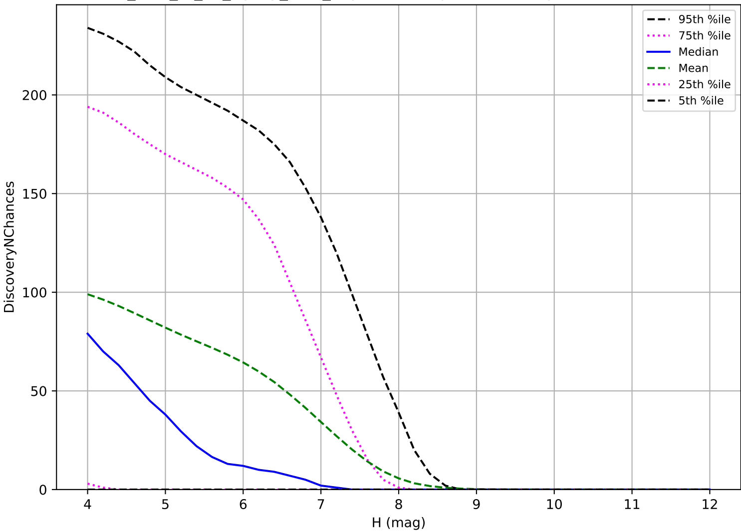
too_elab_r8_d3_ugrizy_v3.4_10yrs: TNO 3 pairs in 15 nights detection loss
