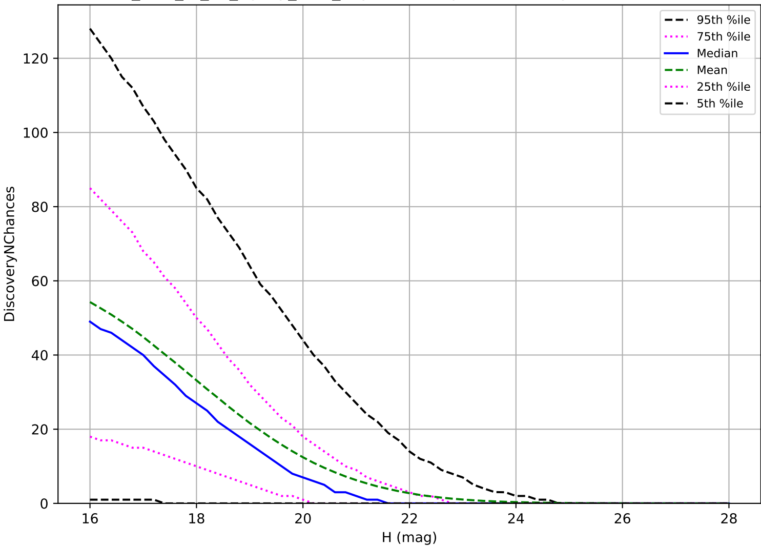
too_elab_r8_d3_ugrizy_v3.4_10yrs: PHA 3 pairs in 15 nights detection loss
