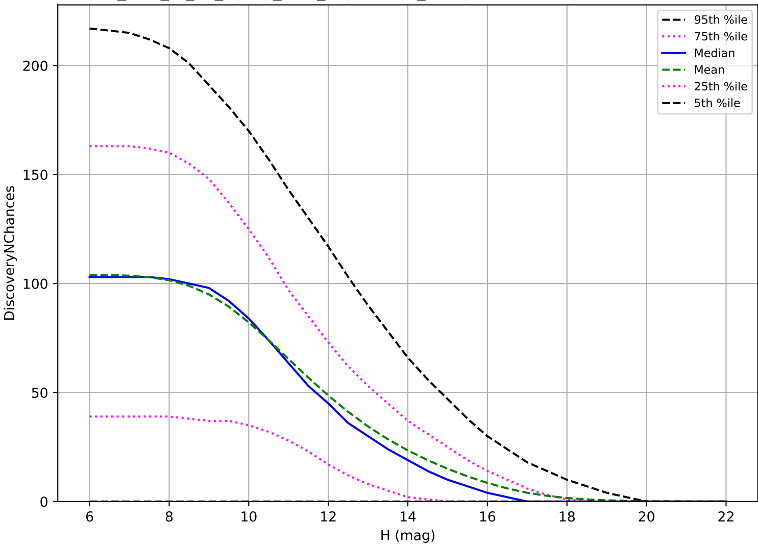
too_elab_r8_d3_ugrizy_v3.4_10yrs: OCC_r5 3 pairs in 15 nights detection loss
