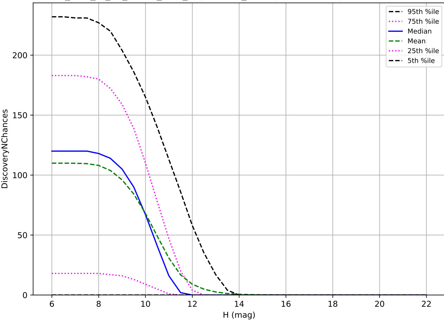
too_elab_r8_d3_ugrizy_v3.4_10yrs: OCC_r20 3 pairs in 15 nights detection loss
