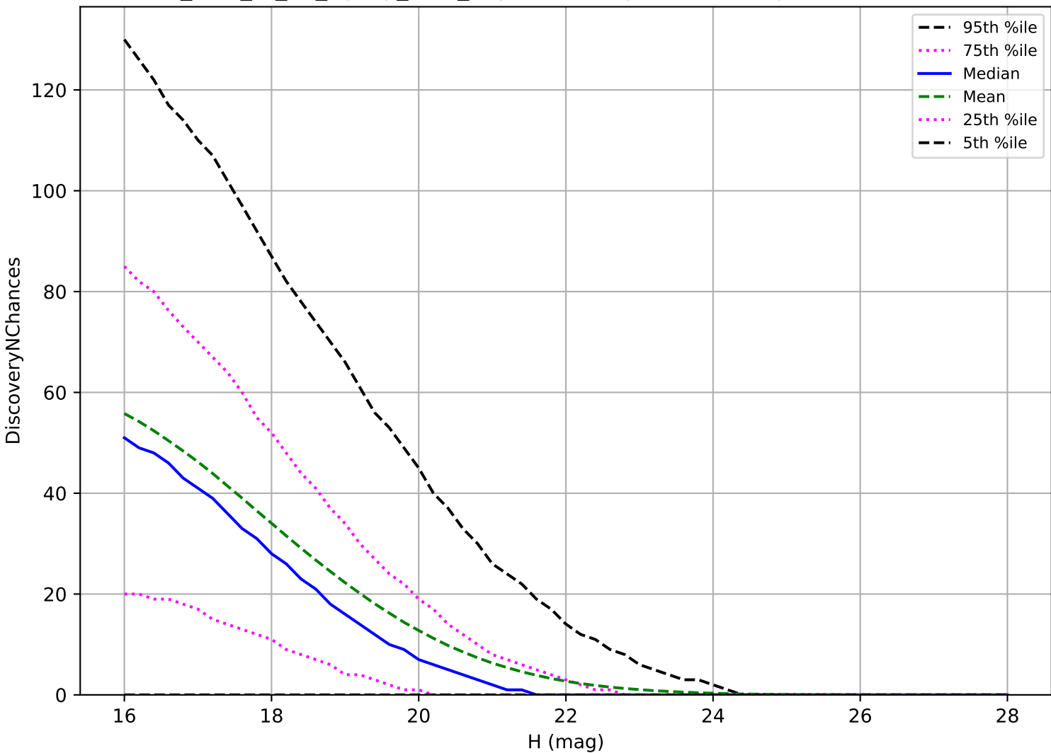
too_elab_r8_d3_ugrizy_v3.4_10yrs: NEO 3 pairs in 15 nights detection loss
