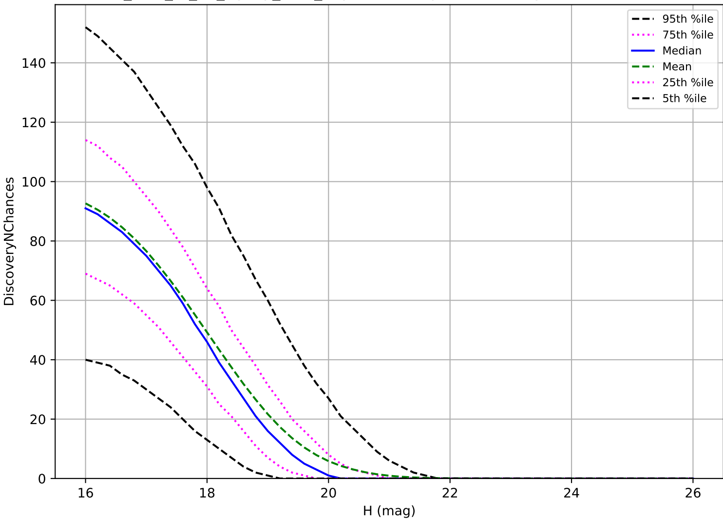
too_elab_r8_d3_ugrizy_v3.4_10yrs: MBA 3 pairs in 15 nights detection loss
