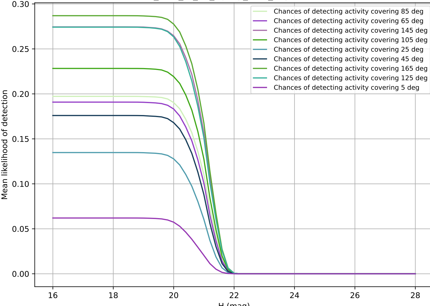
too elab r8 d3 ugrizy v3.4 10yrs Vatira
