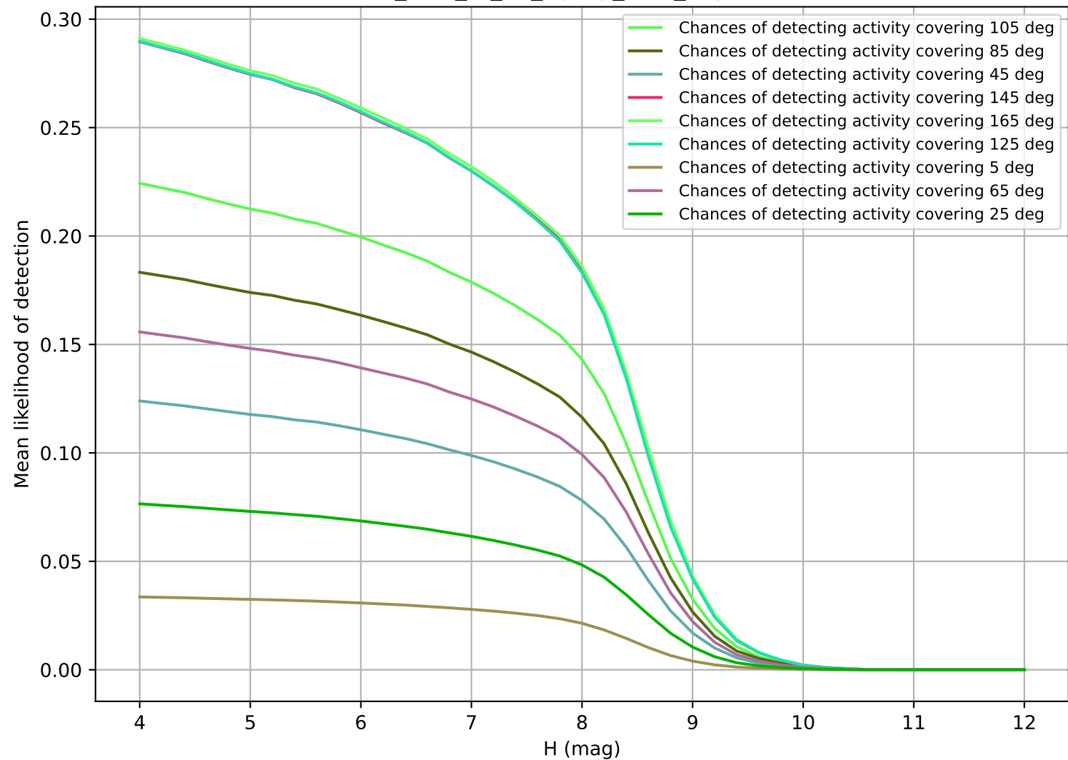
too_elab_r8_d3_ugrizy_v3.4_10yrs TNO
