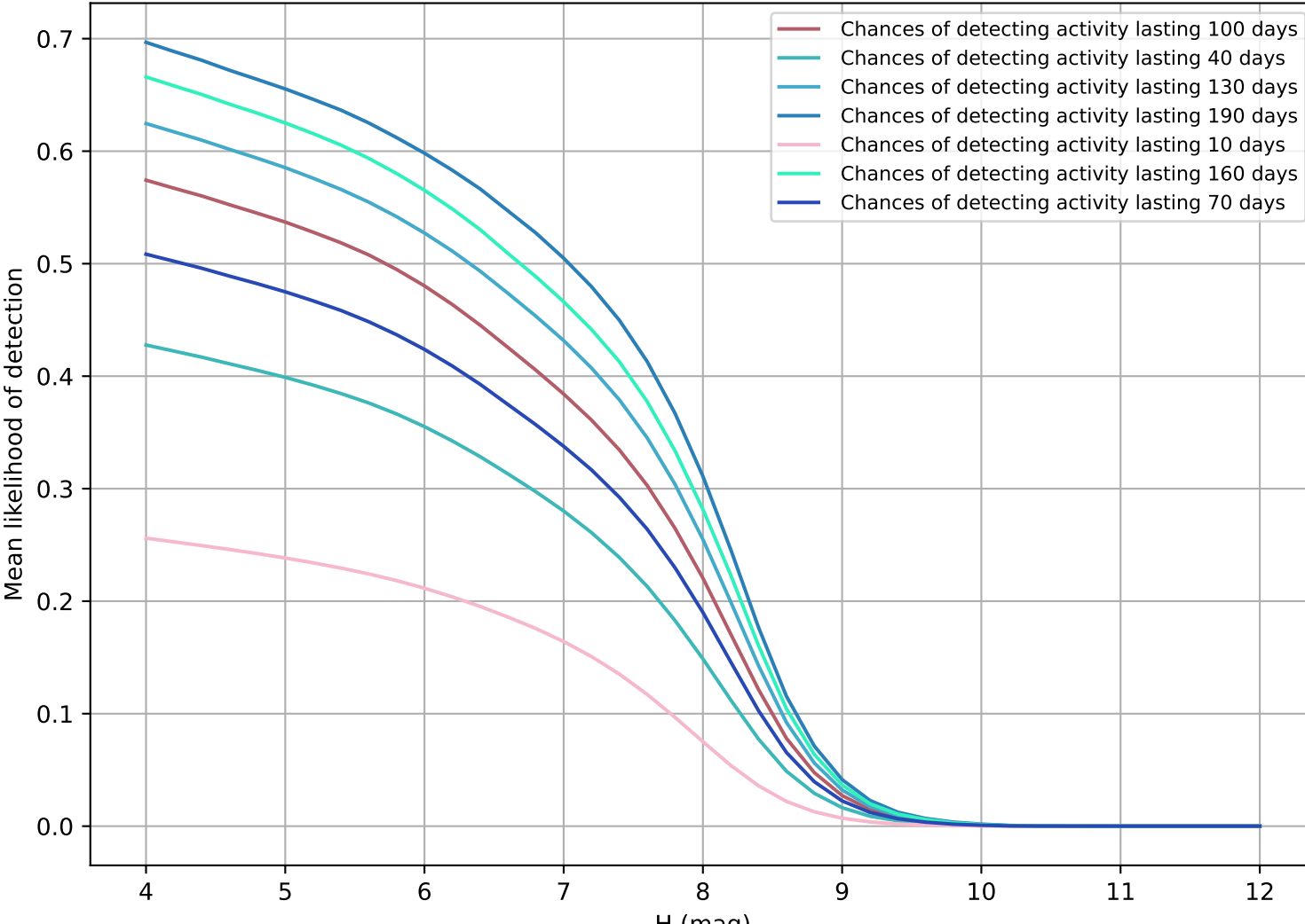
too elab r8 d3 ugrizy v3.4 10yrs TNO
