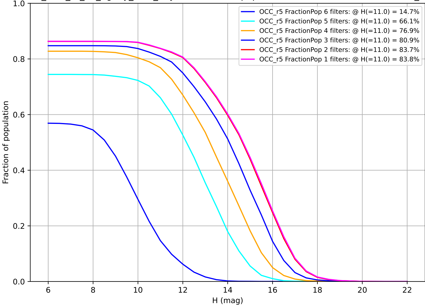
too_elab_r8_d3_ugrizy_v3.4_10yrs: Fraction of population with colors in X filters OCC_r5
