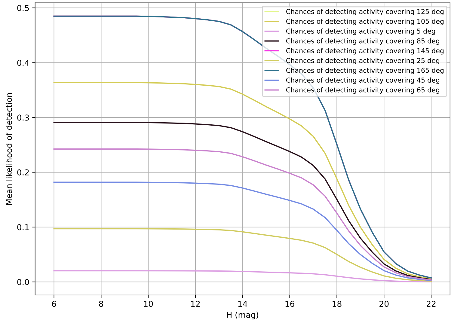
too_elab_r8_d3_ugrizy_v3.4_10yrs OCC_r5
