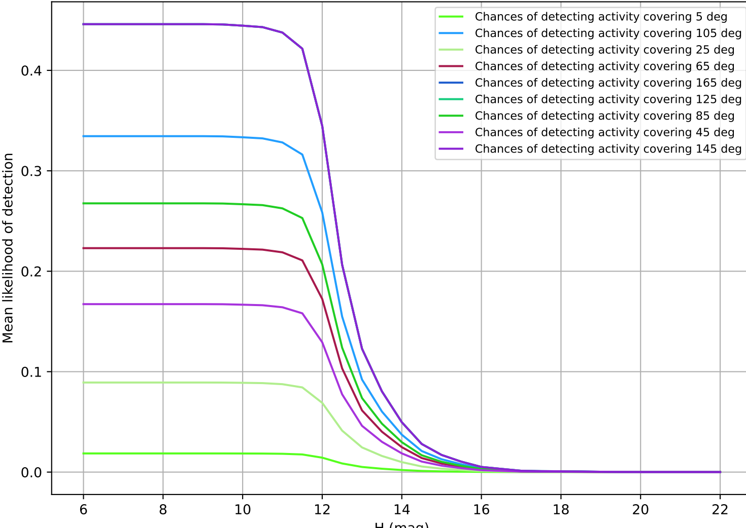
too_elab_r8_d3_ugrizy_v3.4_10yrs OCC_r20
