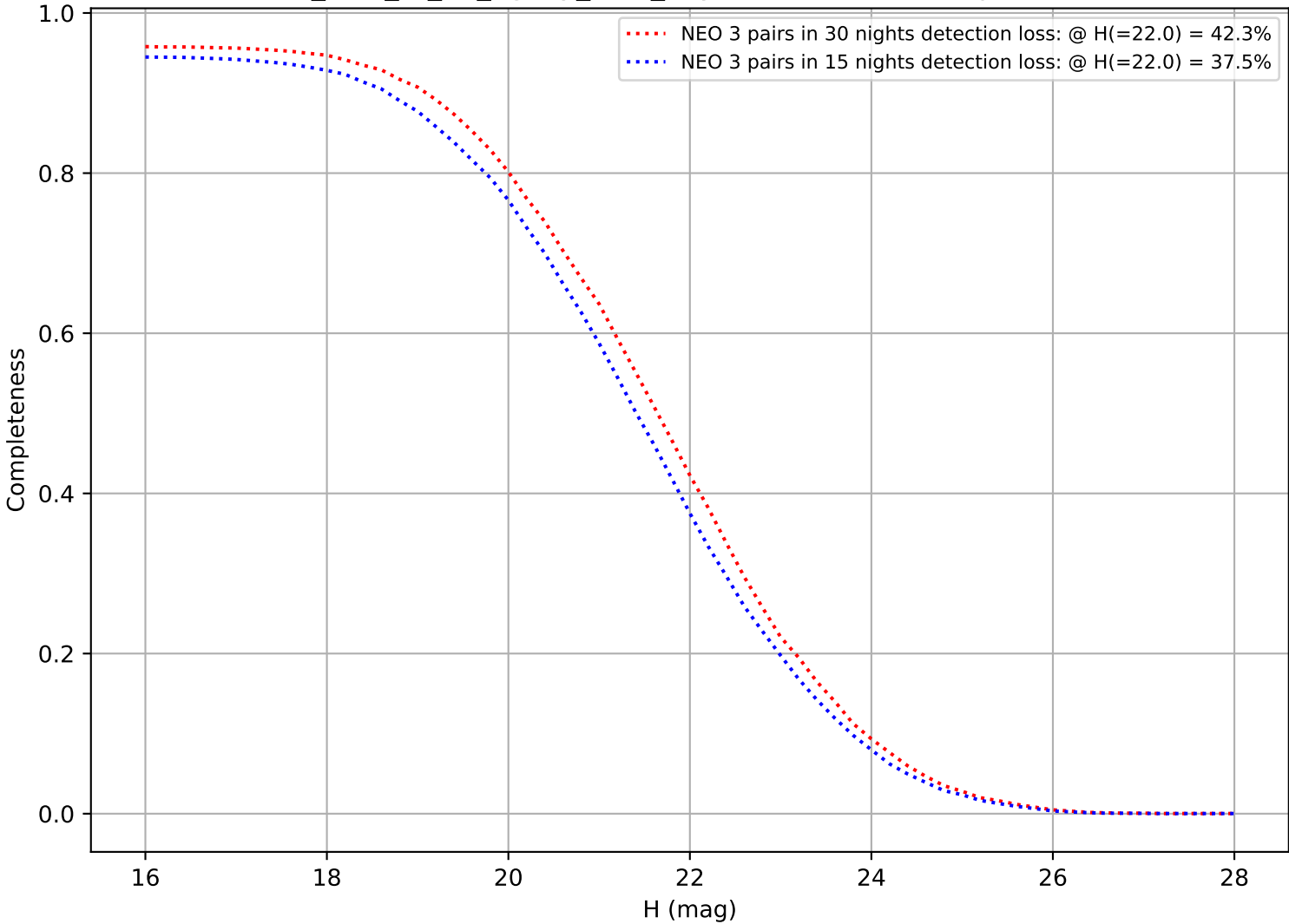
too_elab_r8_d3_ugrizy_v3.4_10yrs: DifferentialCompleteness
