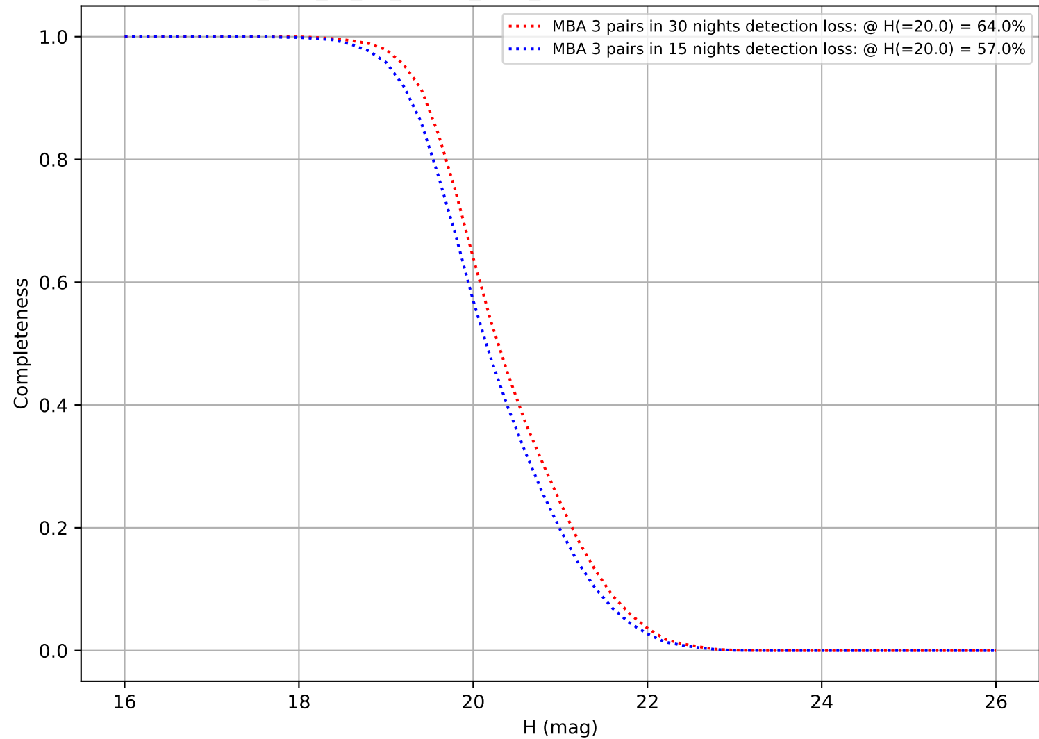
too_elab_r8_d3_ugrizy_v3.4_10yrs: DifferentialCompleteness
