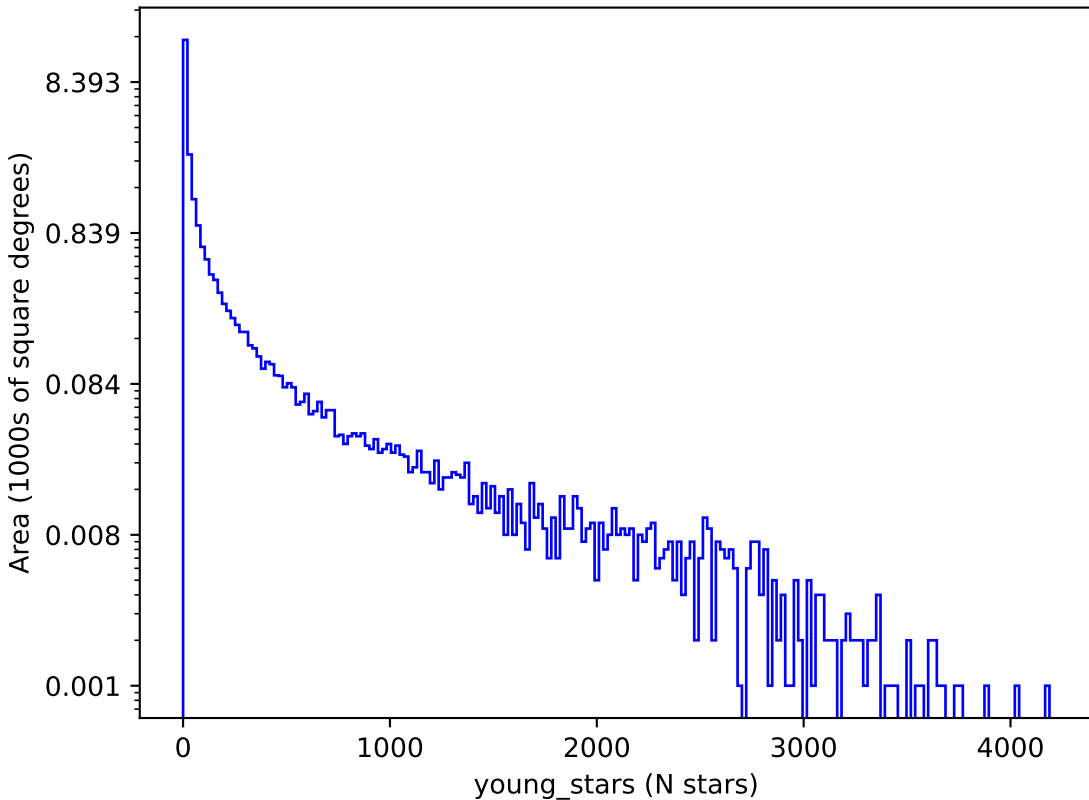
too_elab_r8_d3_ugrizy_v3.4_10yrs : young_stars
