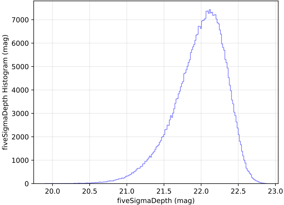
too_elab_r8_d3_ugrizy_v3.4_10yrs y: fiveSigmaDepth Histogram
