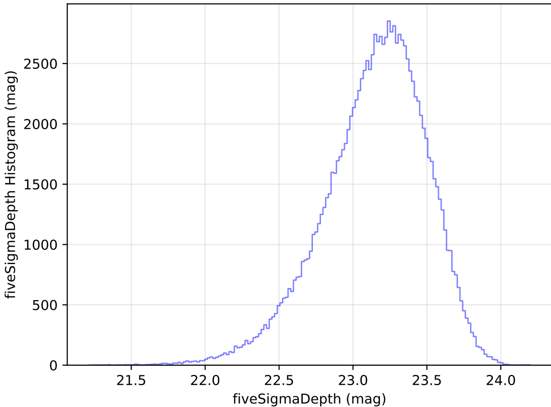
too_elab_r8_d3_ugrizy_v3.4_10yrs u: fiveSigmaDepth Histogram
