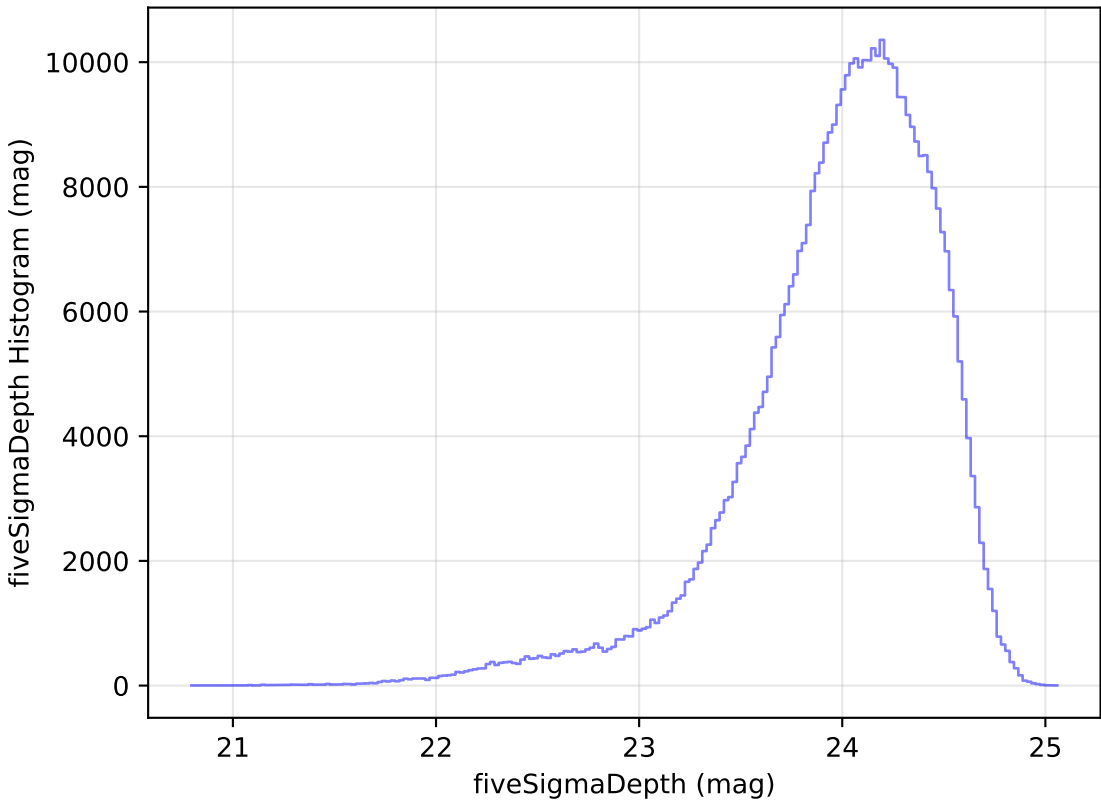
too_elab_r8_d3_ugrizy_v3.4_10yrs r: fiveSigmaDepth Histogram
