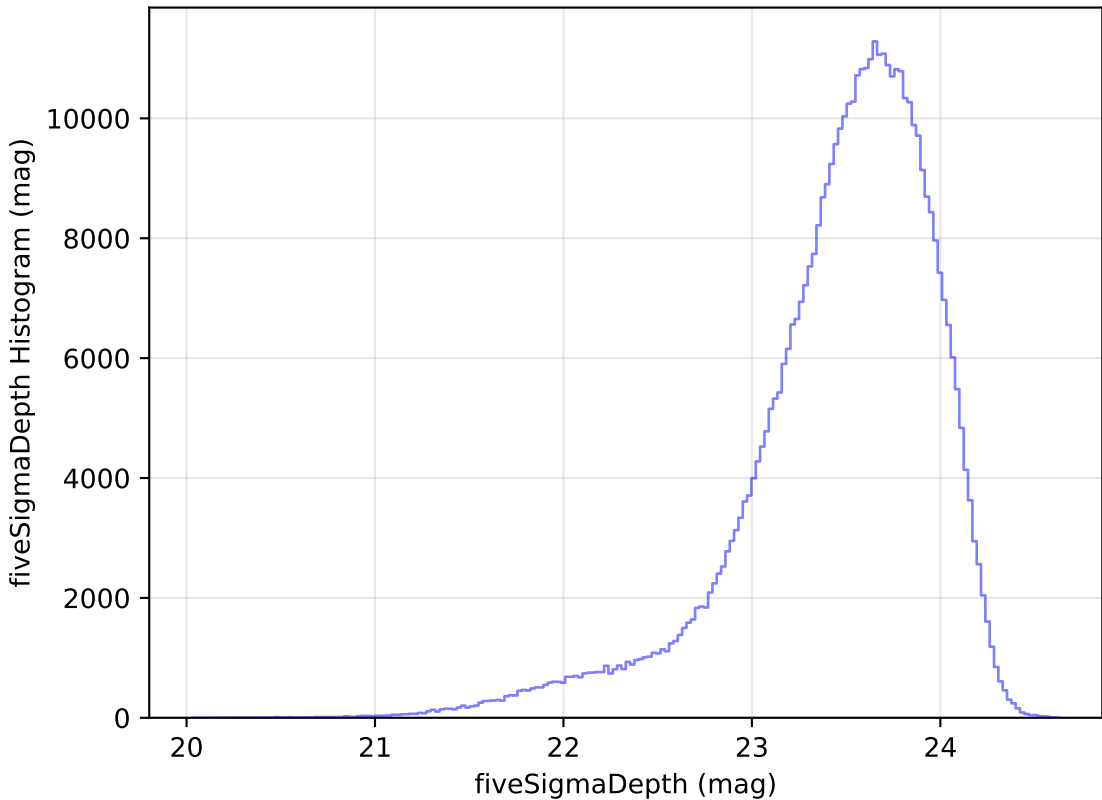
too_elab_r8_d3_ugrizy_v3.4_10yrs i: fiveSigmaDepth Histogram
