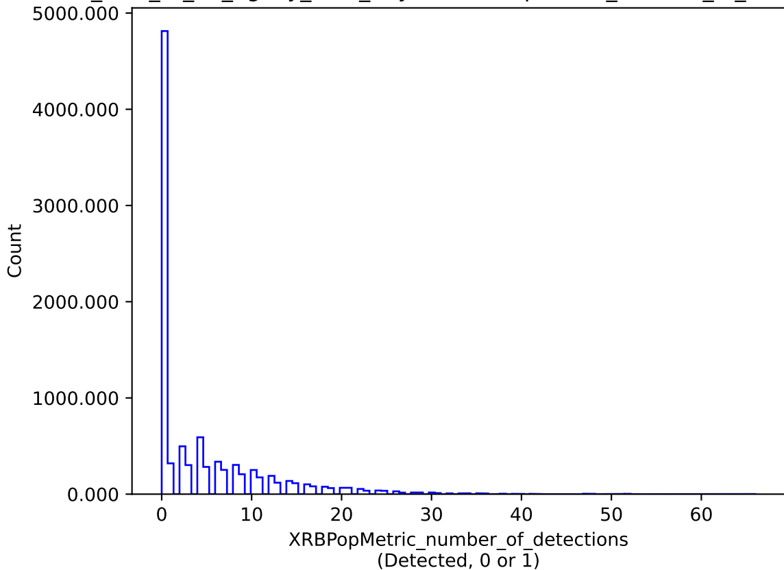
too_elab_r8_d3_ugrizy_v3.4_10yrs : XRBPoMetric_number_of_detections
