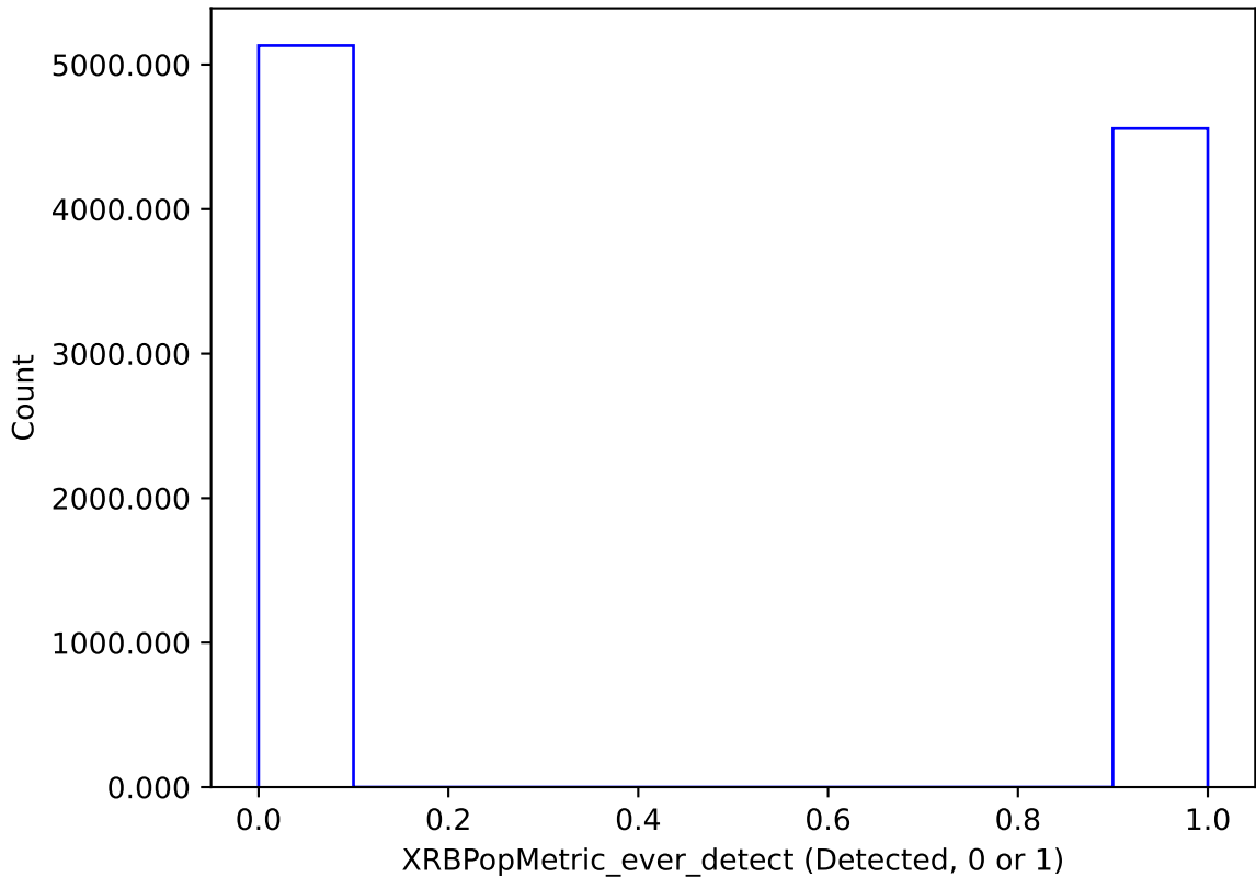
too_elab_r8_d3_ugrizy_v3.4_10yrs : XRBPoMetric_ever_detect
