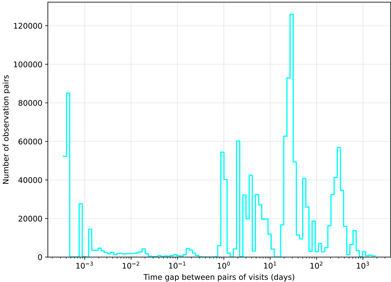
too_elab_r8_d3_ugrizy_v3.4_10yrs u band: Tgaps observationStartMJD
