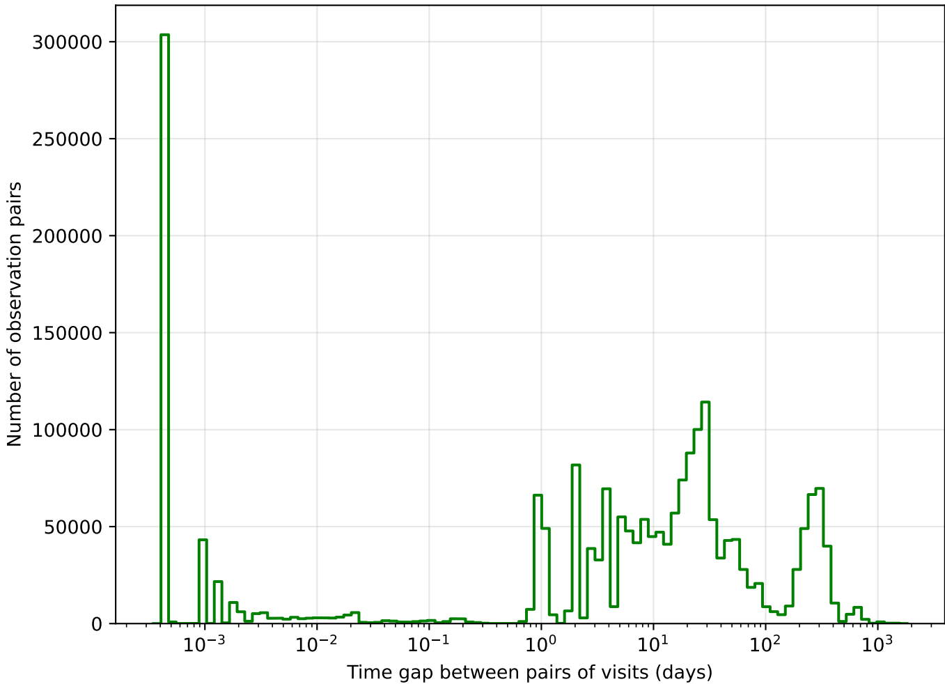
too_elab_r8_d3_ugrizy_v3.4_10yrs g band: Tgaps observationStartMJD
