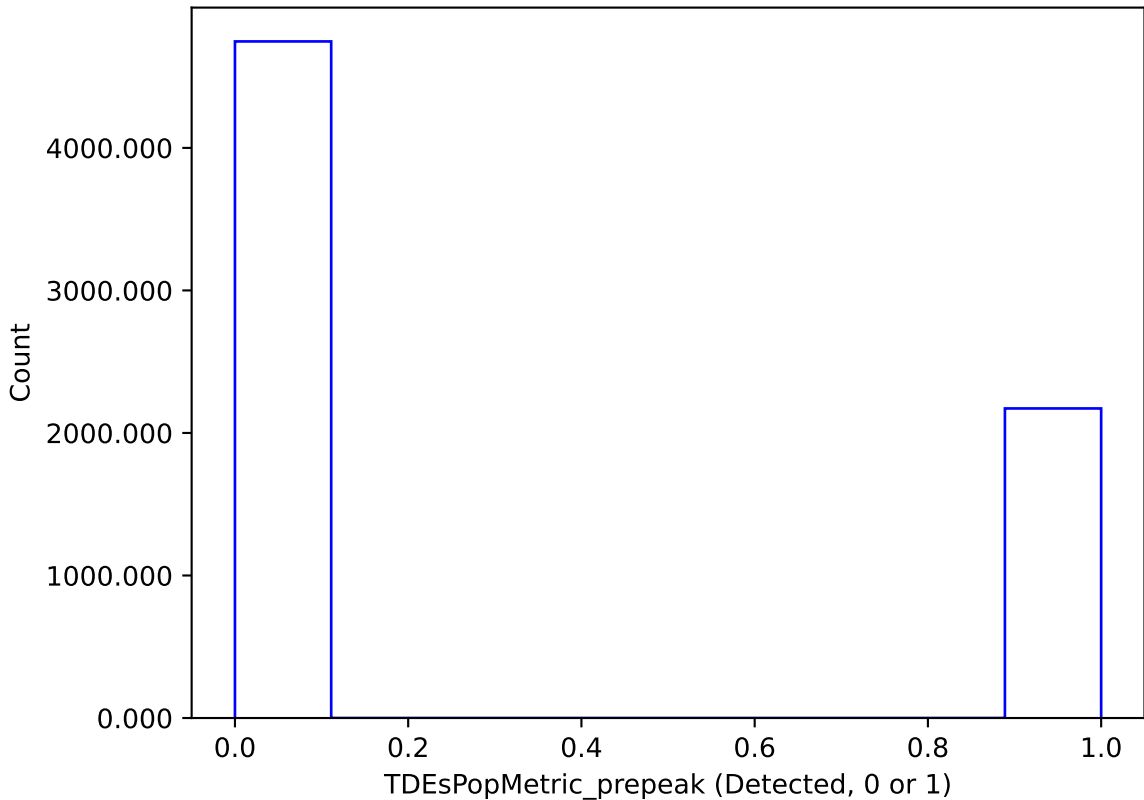
too_elab_r8_d3_ugrizy_v3.4_10yrs : TDEsPopMetric_prepeak
