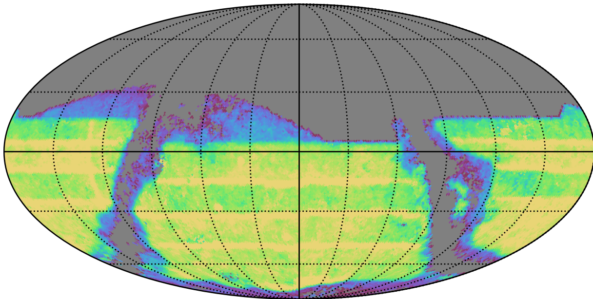
too_elab_r8_d3_ugrizy_v3.4_10yrs : TDC_rate
