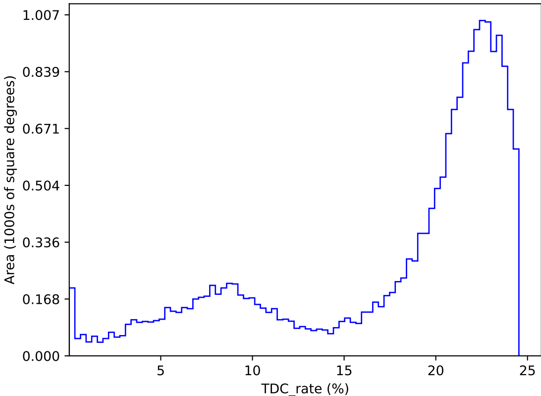
too_elab_r8_d3_ugrizy_v3.4_10yrs : TDC_rate
