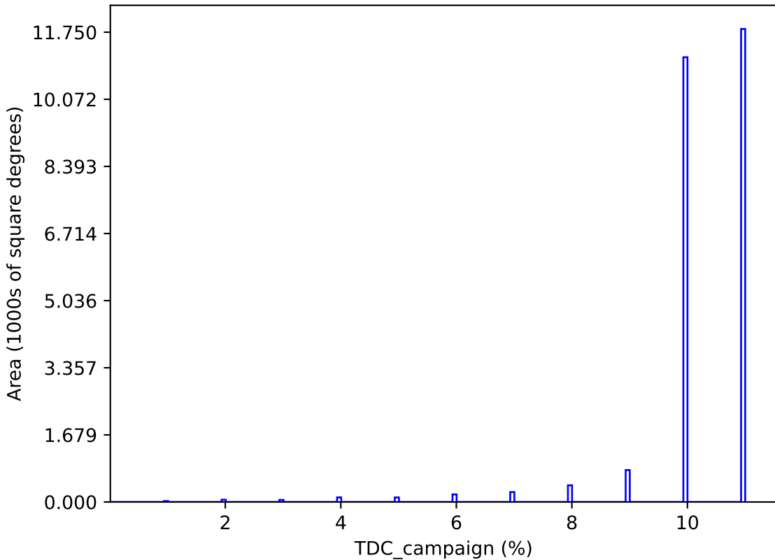
too_elab_r8_d3_ugrizy_v3.4_10yrs : TDC_campaign
