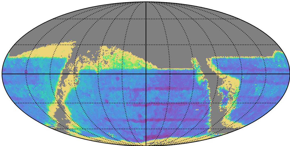
too_elab_r8_d3_ugrizy_v3.4_10yrs : TDC_accuracy
