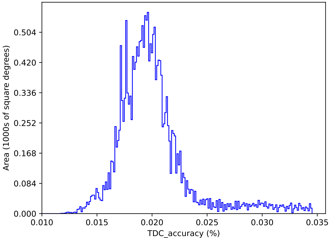
too_elab_r8_d3_ugrizy_v3.4_10yrs : TDC_accuracy
