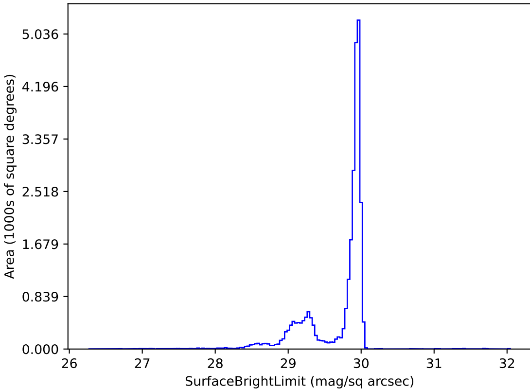
too_elab_r8_d3_ugrizy_v3.4_10yrs i: SurfaceBrightLimit
