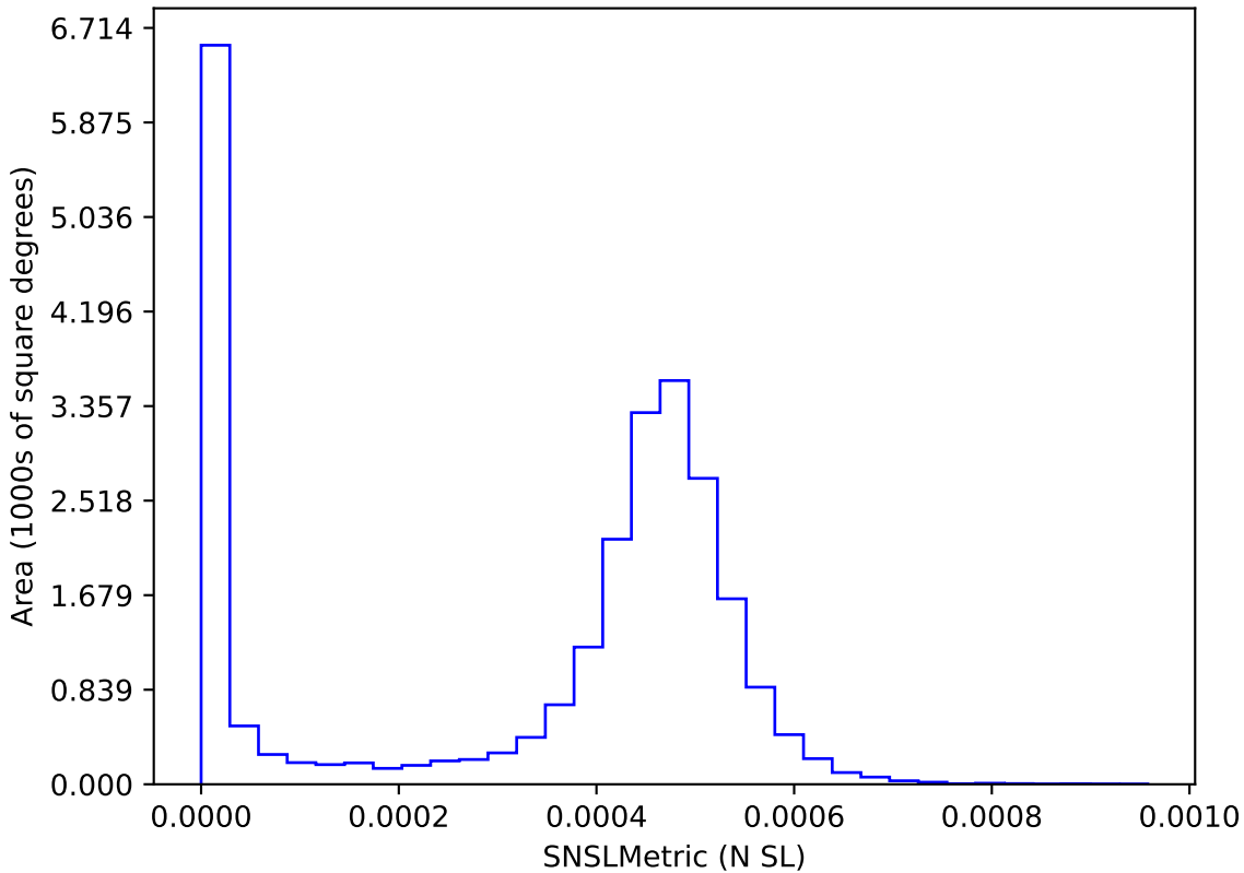
too_elab_r8_d3_ugrizy_v3.4_10yrs : SNSLMetric
