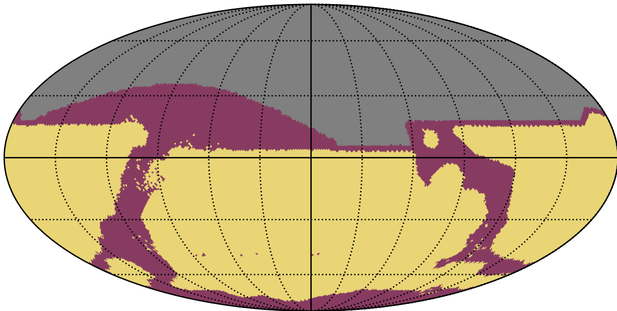
too_elab_r8_d3_ugrizy_v3.4_10yrs : RapidRevisits
