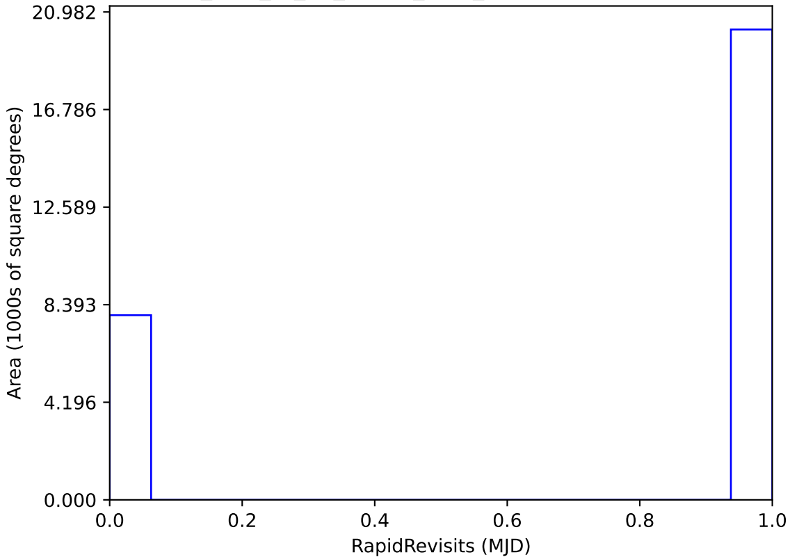
too_elab_r8_d3_ugrizy_v3.4_10yrs : RapidRevisits
