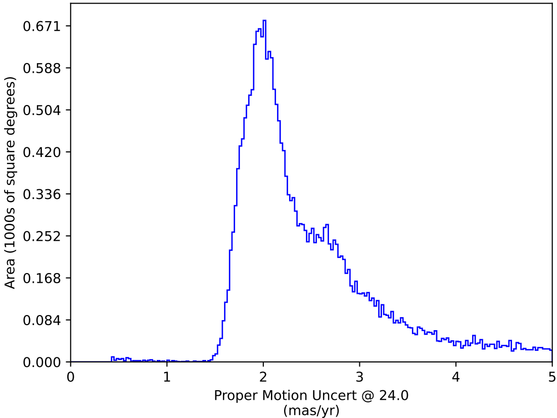
too_elab_r8_d3_ugrizy_v3.4_10yrs : Proper Motion Uncert @ 24.0
