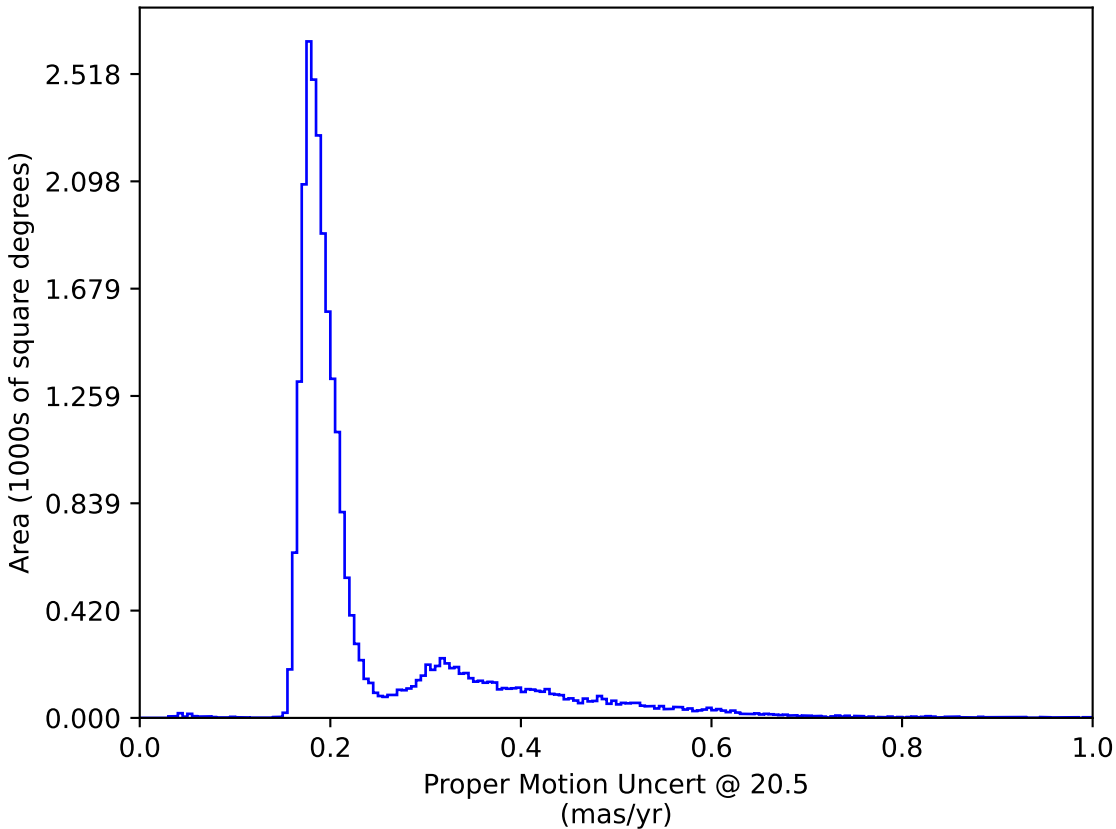
too_elab_r8_d3_ugrizy_v3.4_10yrs : Proper Motion Uncert @ 20.5
